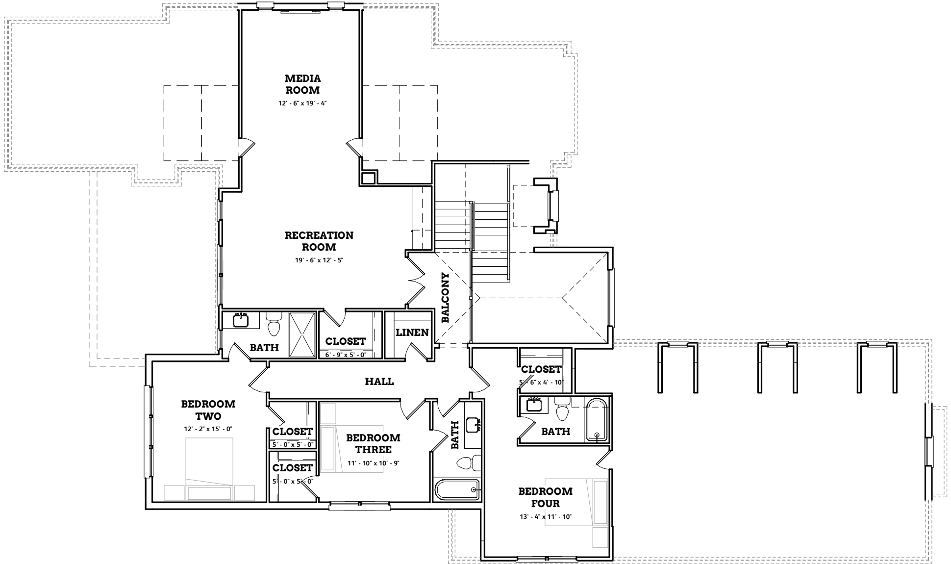
SECOND FLOOR
