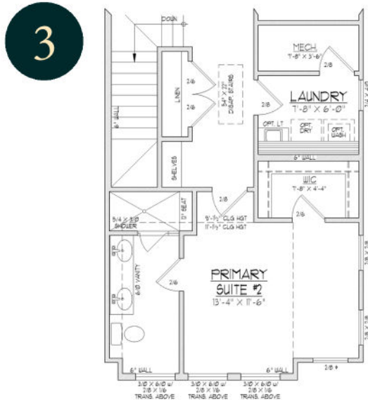
THIRD FLOOR PLAN B w/ OPT. DUAL PRIMARY
