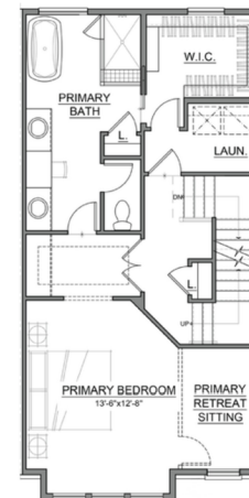
OPT. SECOND FLOOR PLAN DELUXE PRIMARY
