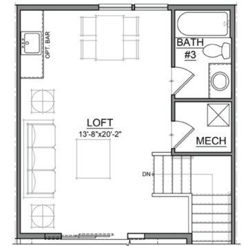
OPT. THIRD FLOOR PLAN EXPANDED LOFT
