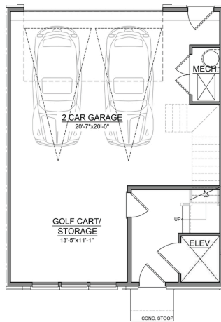
OPT. FIRST FLOOR PLAN 2-CAR GARAGE & GOLF CART BAY
